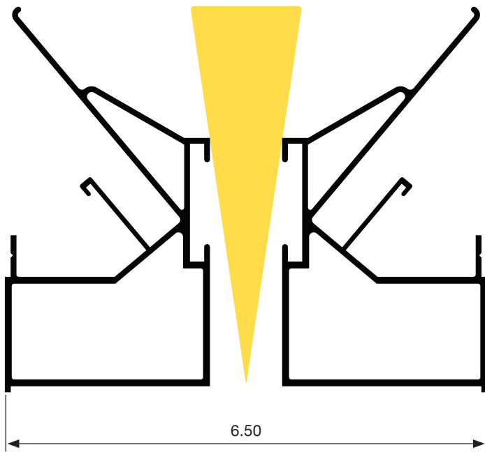
FLEX INTEGRATED FRAME
