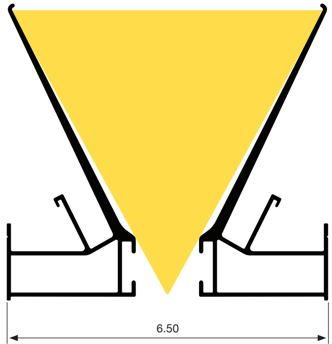
FLEX INTEGRATED 2.0 FRAME
