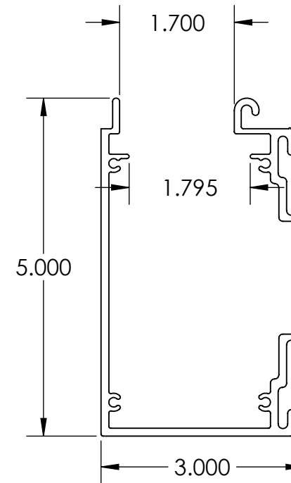
PROFILE VIEW
