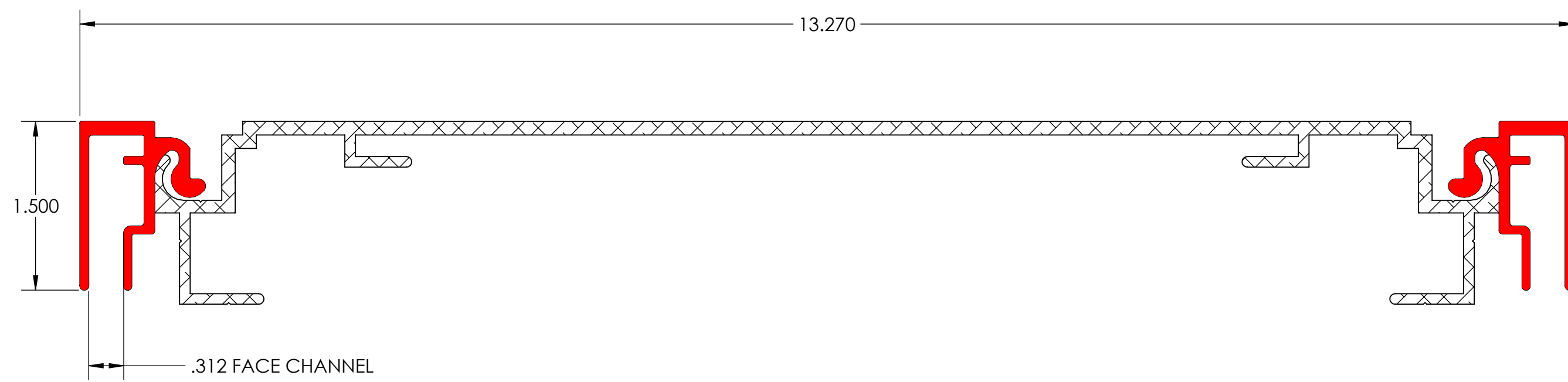
SECTION A-A ESP-12 HINGED FRAME WITH ESP-F HINGED RETAINERS SCALE 1 : 1
