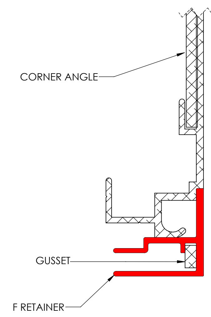
SECTION B-B ESP-12 HINGED FRAME WITH ESP-F RETAINERS SCALE 1 : 1
