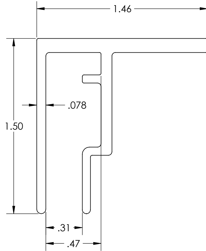
PROFILE VIEW
