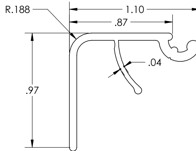
PROFILE VIEW SCALE 2:1
