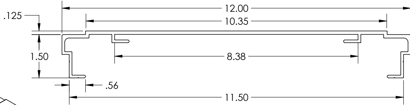
PROFILE VIEW
